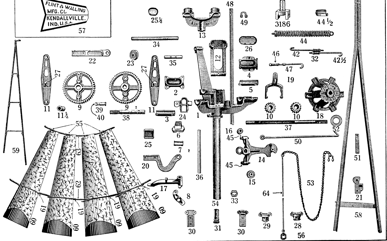
Repair Chart Fig. 606 Model 12 Star Windmill
